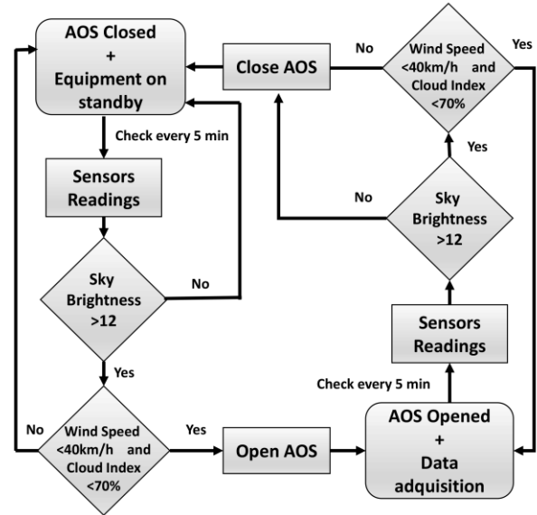
Figure 1. Flow diagram for data acquisition and operation of the observatory.
