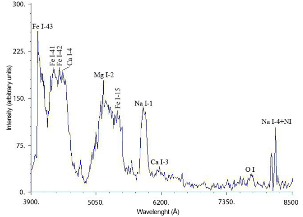
Figure 3. Emission spectrum of meteor M20160727_022352 in units of relative intensity as a function of wavelength (Å).
