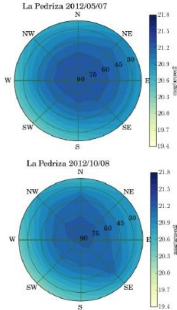
Fig. 1. Sky brightness graphs ( \text{mag}/\text{arcsec}^2 ) obtained with SQM during 2012, at the location where the OAA was later located.
